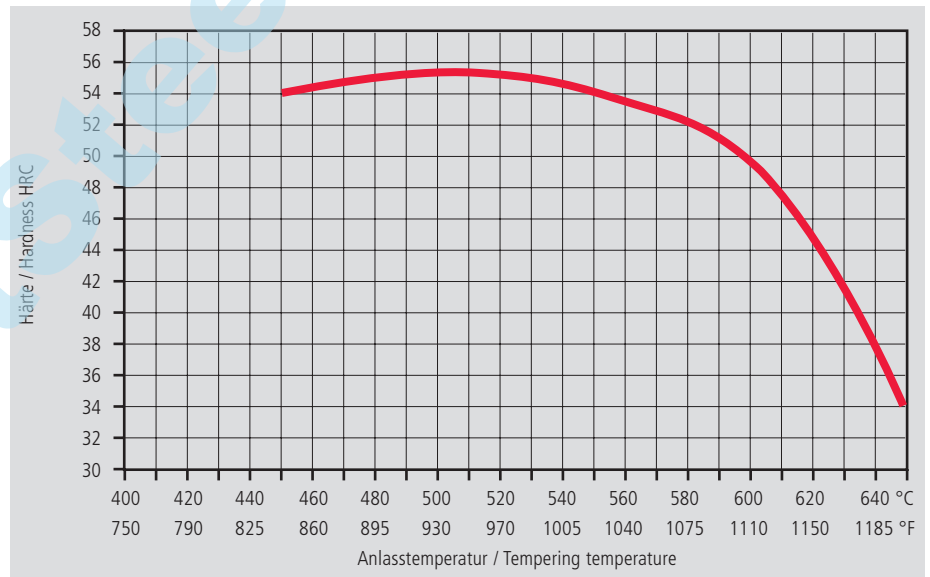
Tempering chart
